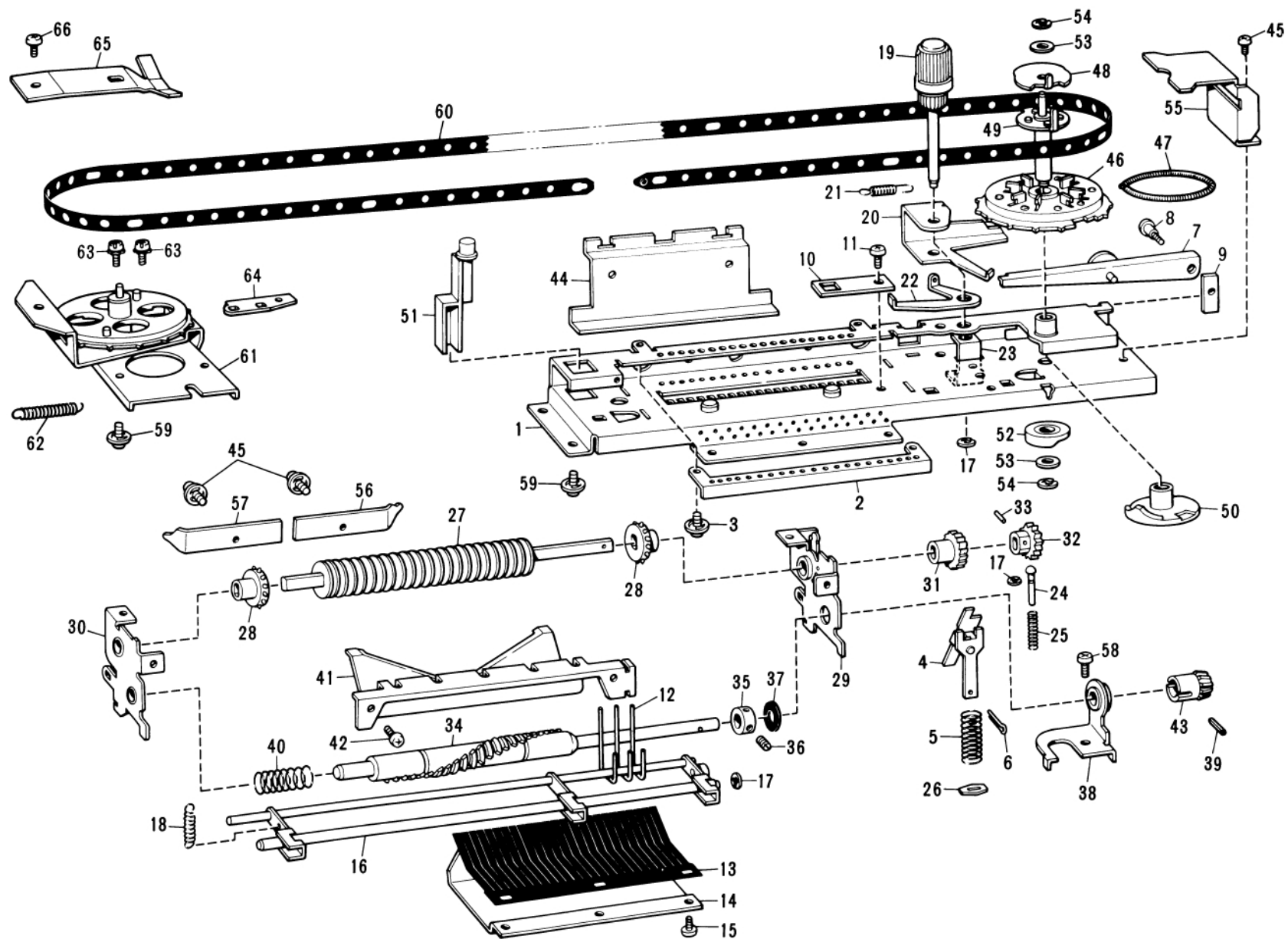
NEEDLE SELECTOR UNIT
