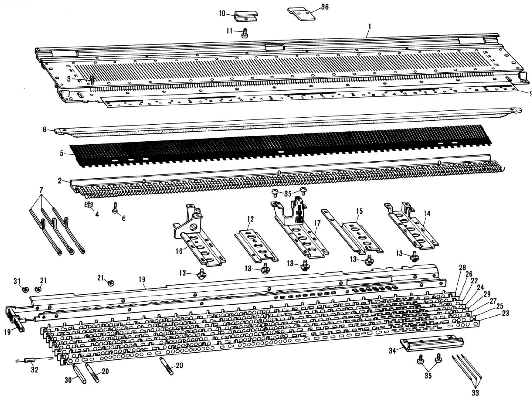
PARTS FOR NEEDLE BED
