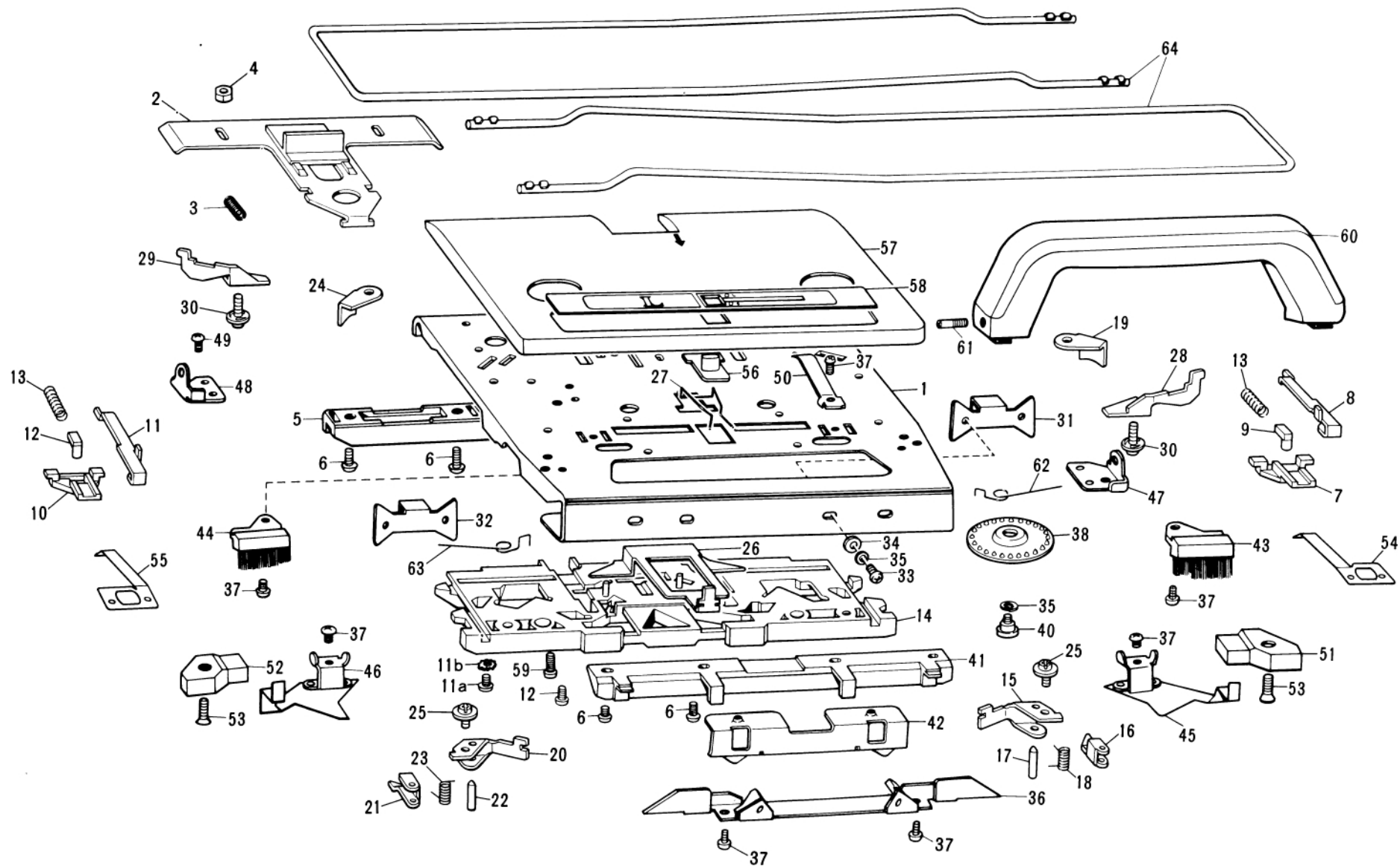
PARTS FOR L-CARRIAGE
