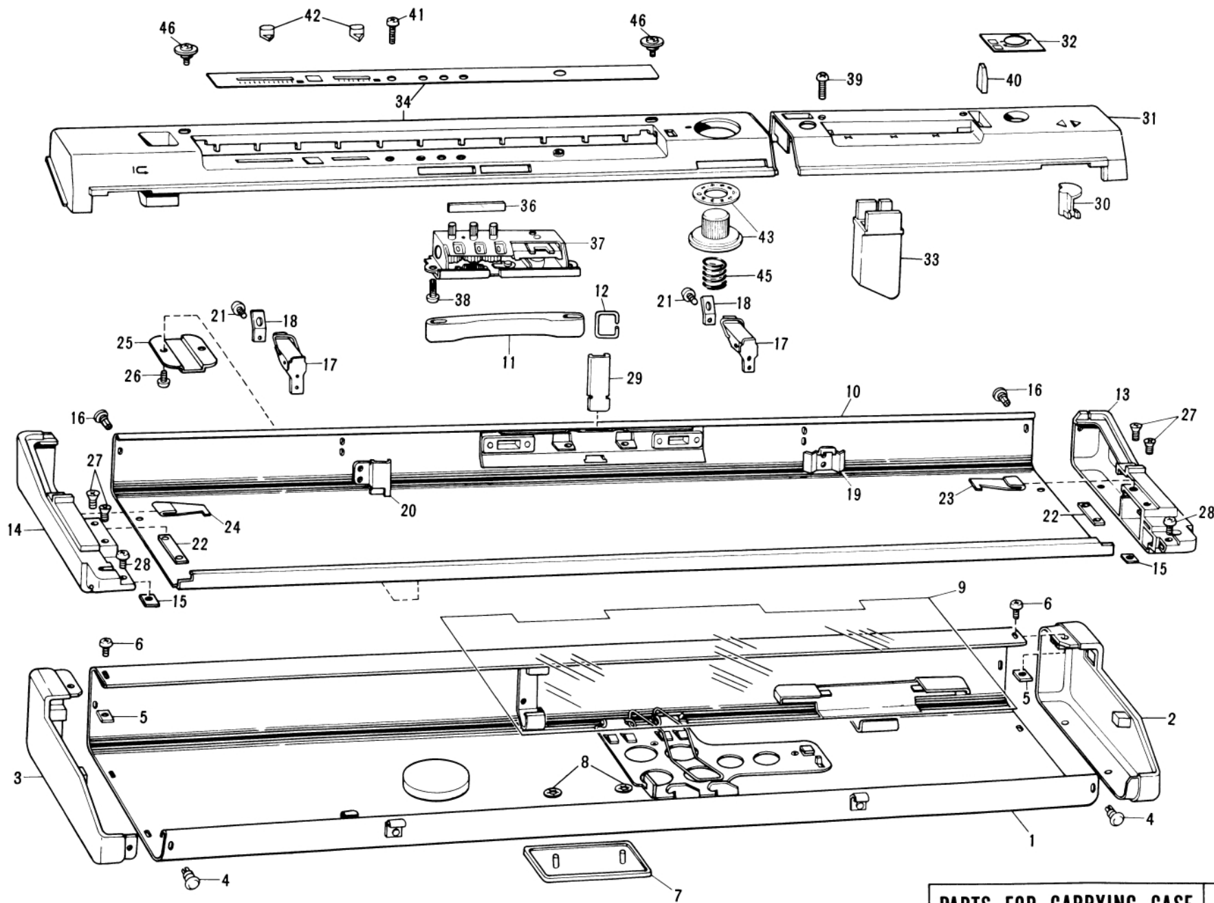
PARTS FOR CARRYING CASE Fig : D
